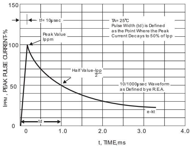
FIGURE 3-PULSE WAVEFORM
