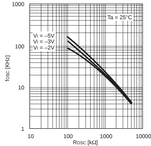
Clock frequency vs. External resistance
