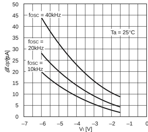
Multiplier current vs. Input voltage
