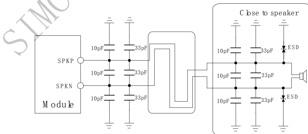
Figure 30: Speaker reference circuit
