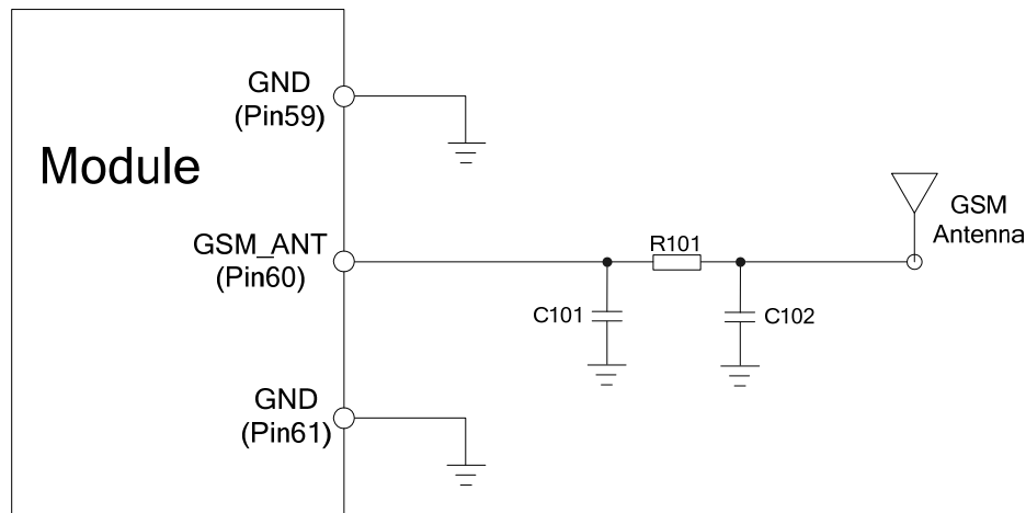
Figure 49: GSM simple antenna matching circuit
