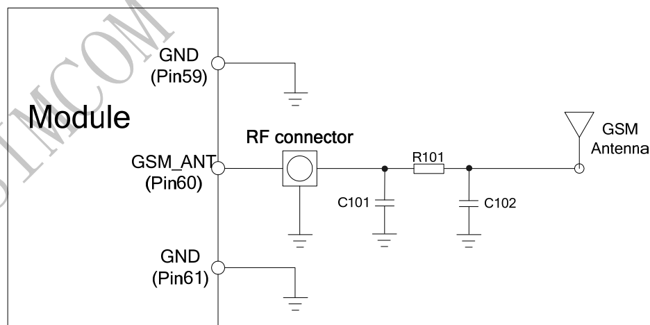
Figure 48: GSM antenna matching circuit
