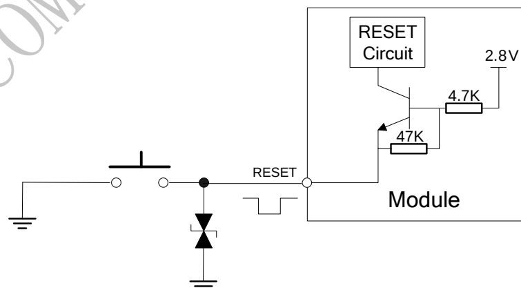
Figure 14: Reset circuit
