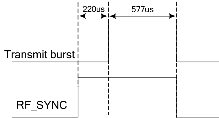
Figure 47: RF_SYNC signal during transmit burst
