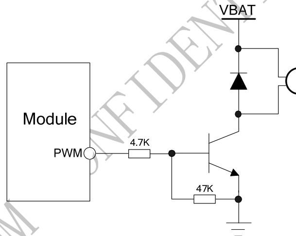
Figure 44: Reference circuit of PWM drive buzzer
