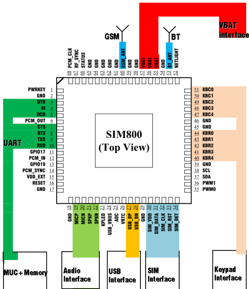
Figure 51: Recommended PCB layout
