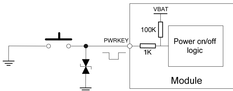
Figure 11: Power on/off module using button
