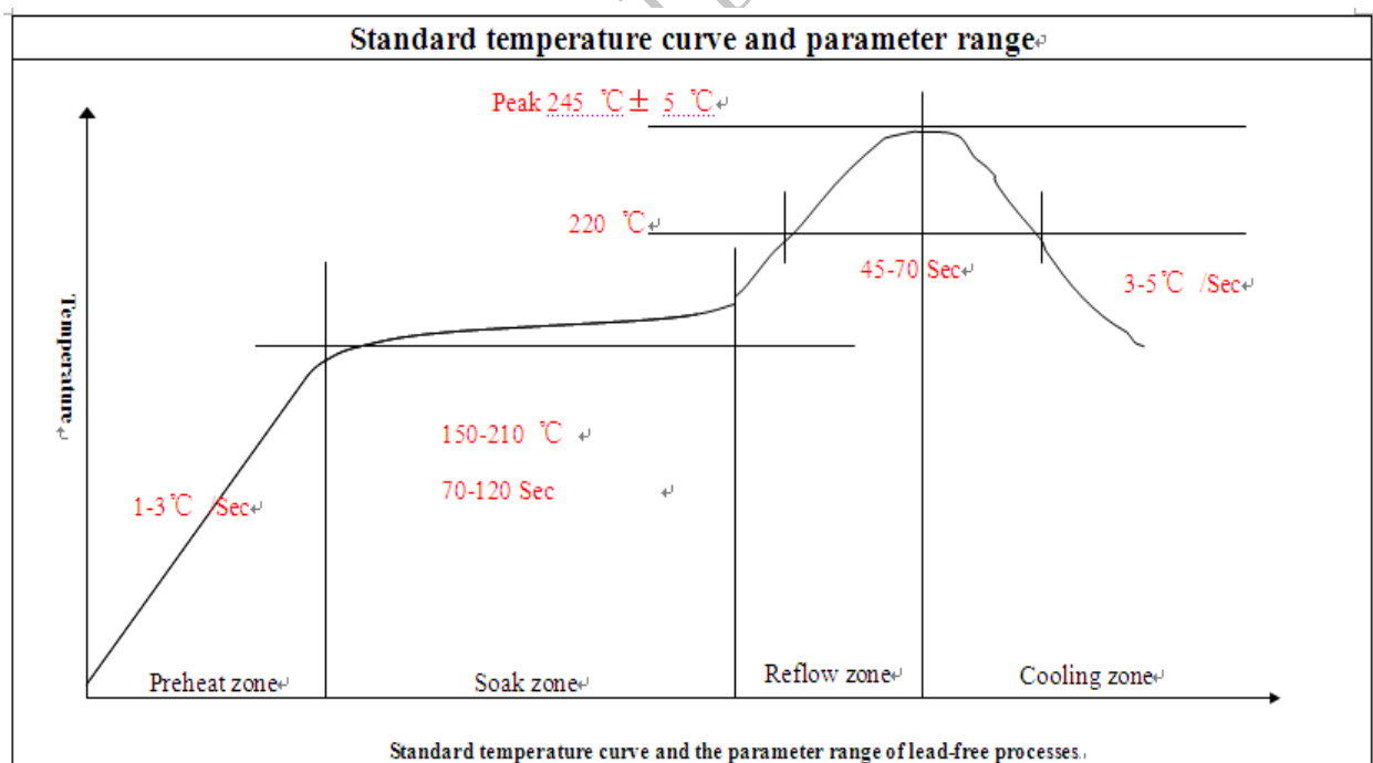
Figure 53: Typical Solder Reflow Profile
