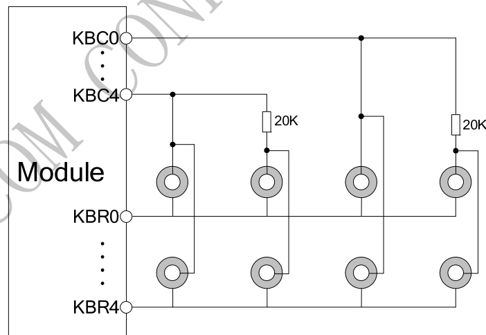
Figure 40: Extended keypad reference circuit
