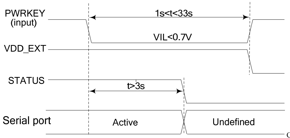
Figure 13: Timing of Power off SIM800 by PWRKEY
