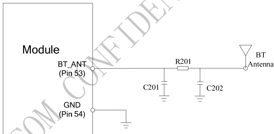
Figure 50: Bluetooth antenna matching circuit
