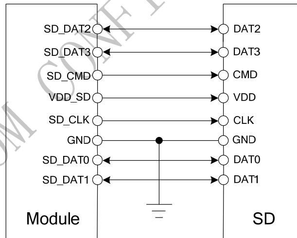
Figure 38: SD reference circuit
