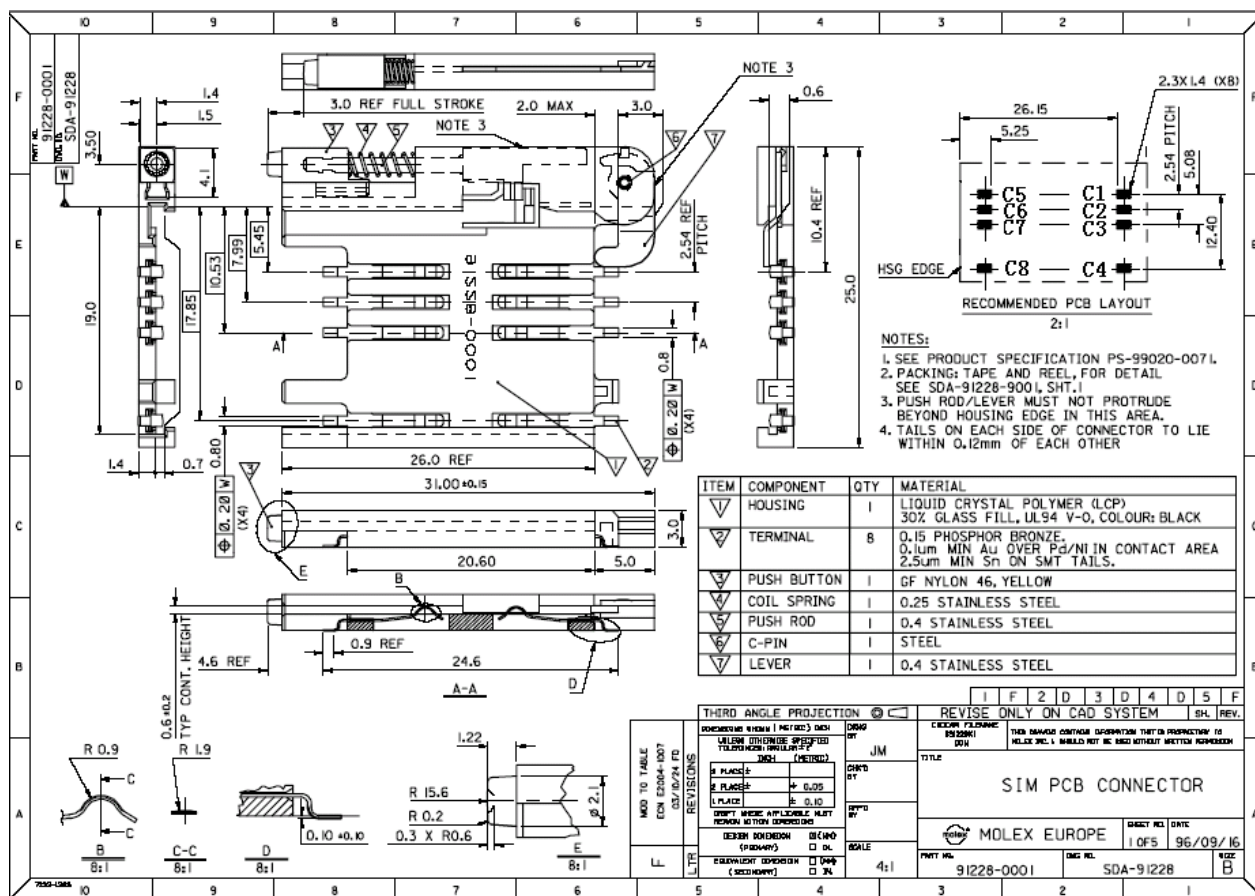
Figure 34: Molex 91228 SIM card holder
