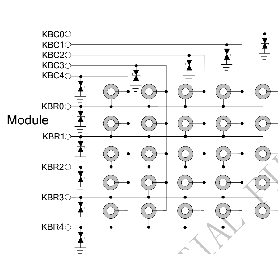
Figure 39: Traditional keypad reference circuit
