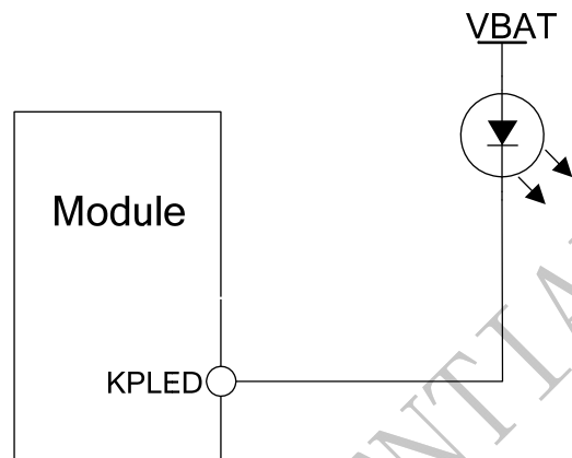
Figure 46: KPLED driver reference circuit
