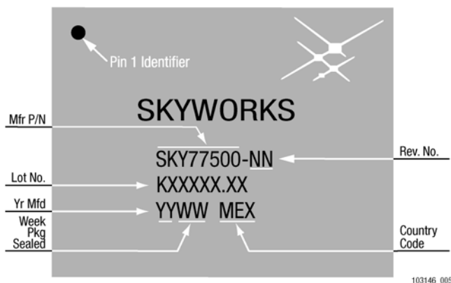
Figure 6. Typical Case Markings
