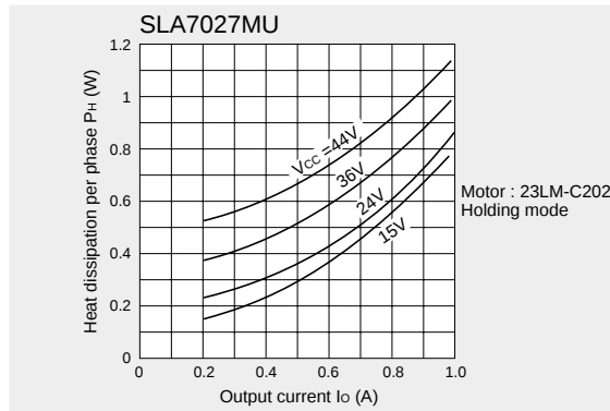
Fig. 7 Heat dissipation per phase P_H vs. Output current I_o
