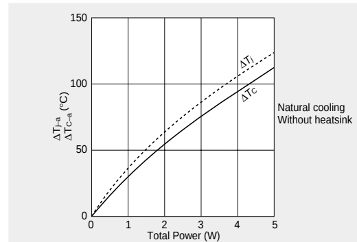
Fig. 8 Temperature rise
