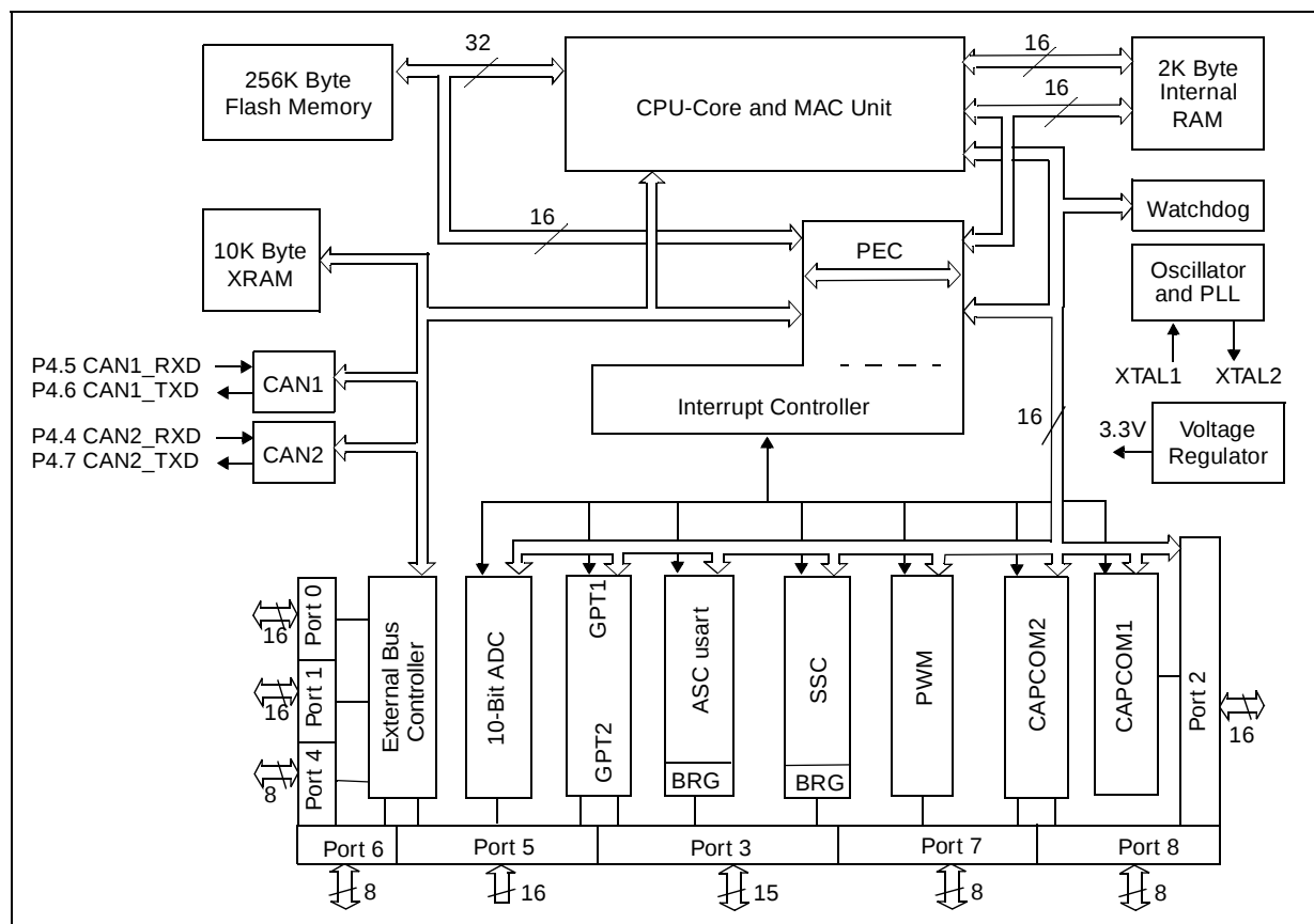
Figure 3 : Block Diagram
