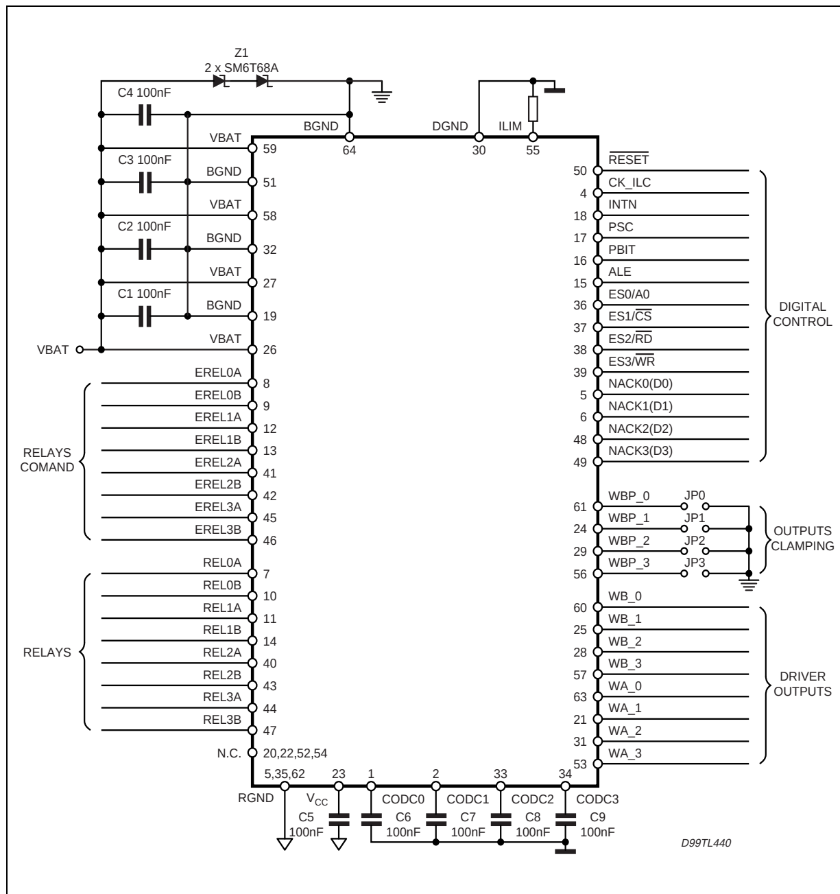
Figure 5. Typical Application Circuit
