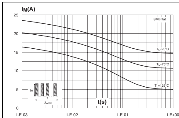
Figure 7. Non repetitive surge peak forward current versus overload duration (maximum values) SMB flat
