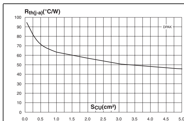
Figure 17. Thermal resistance junction to ambient versus copper surface under each lead (epoxy printed board FR4, e_{CU} = 35 \mu m ) (DPAK)
