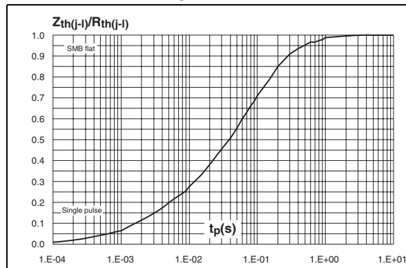
Figure 13. Relative variation of thermal impedance junction to lead versus pulse duration - SMB flat
