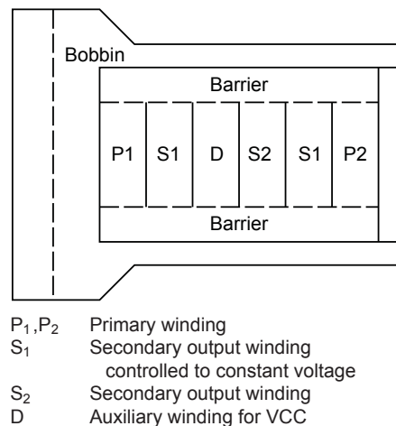
Figure 8. Winding structural example (b)
