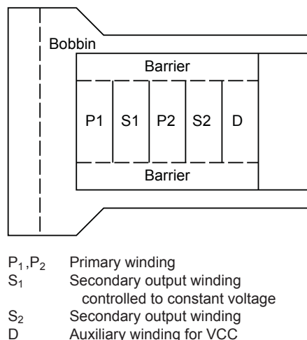
Figure 7. Winding structural example (a)
