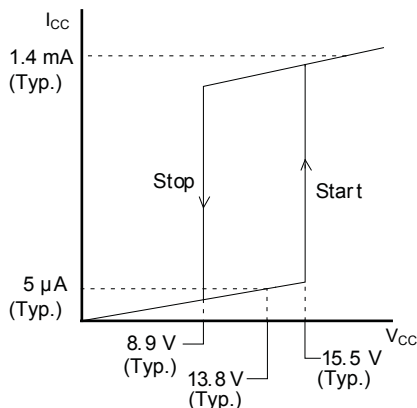
Figure 3. VCC versus ICC
