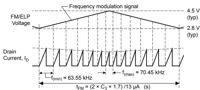
Figure 10. FM/ELP pin voltage and frequency modulation period
