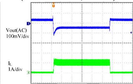
Load Transient ( V_{in}=5.0V , V_{out}=1.8V , I_{load}=0\sim 1A )
