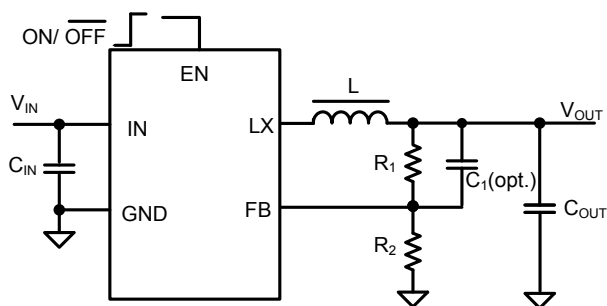
Figure 1. Schematic diagram
