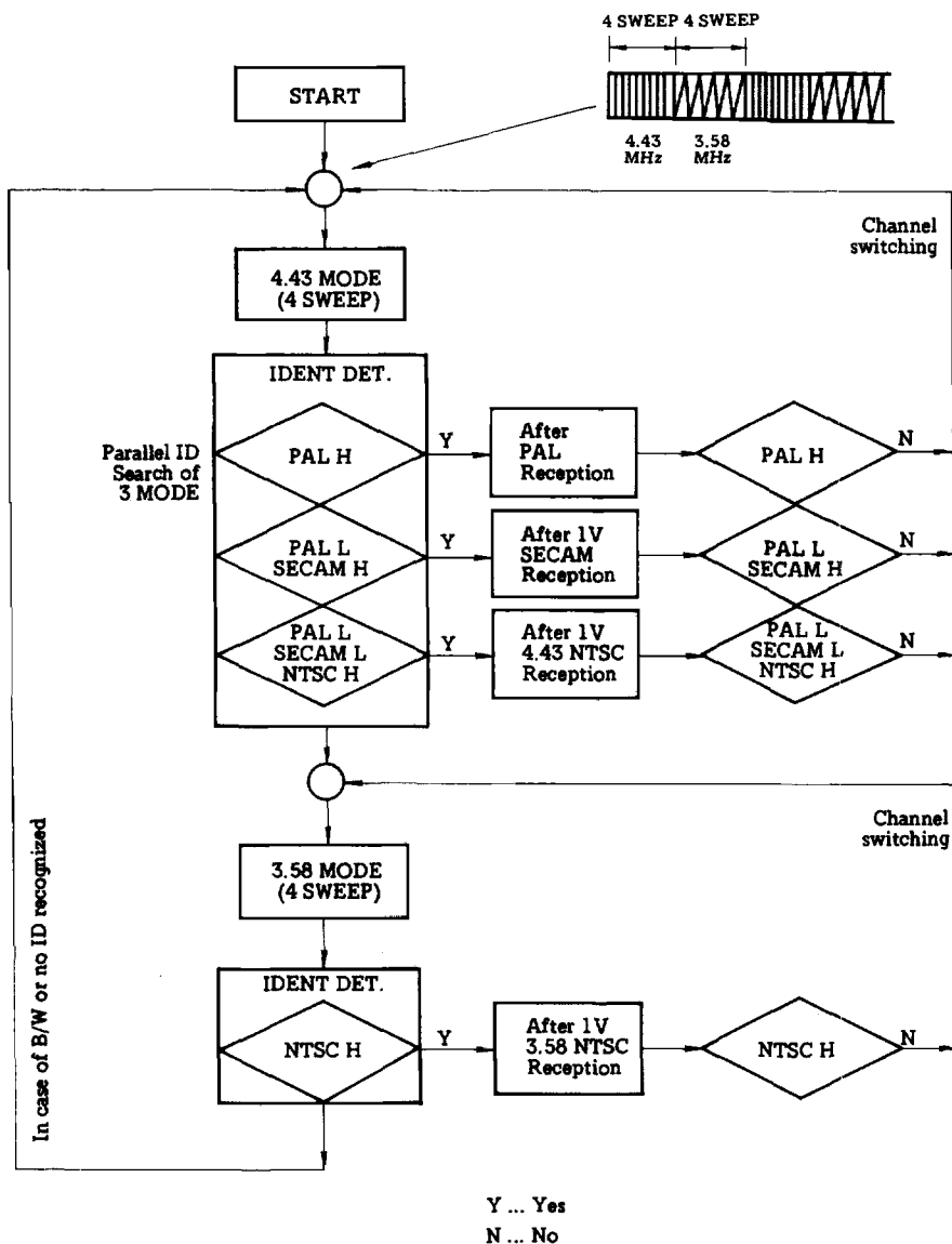
FLOW CHART OF SYSTEM IDENTIFICATION
