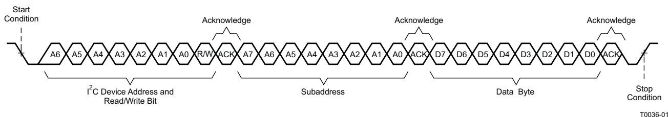
Figure 40. Single-Byte Write Transfer
