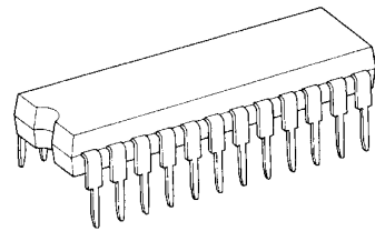
SDIP24-P-300-1.78
