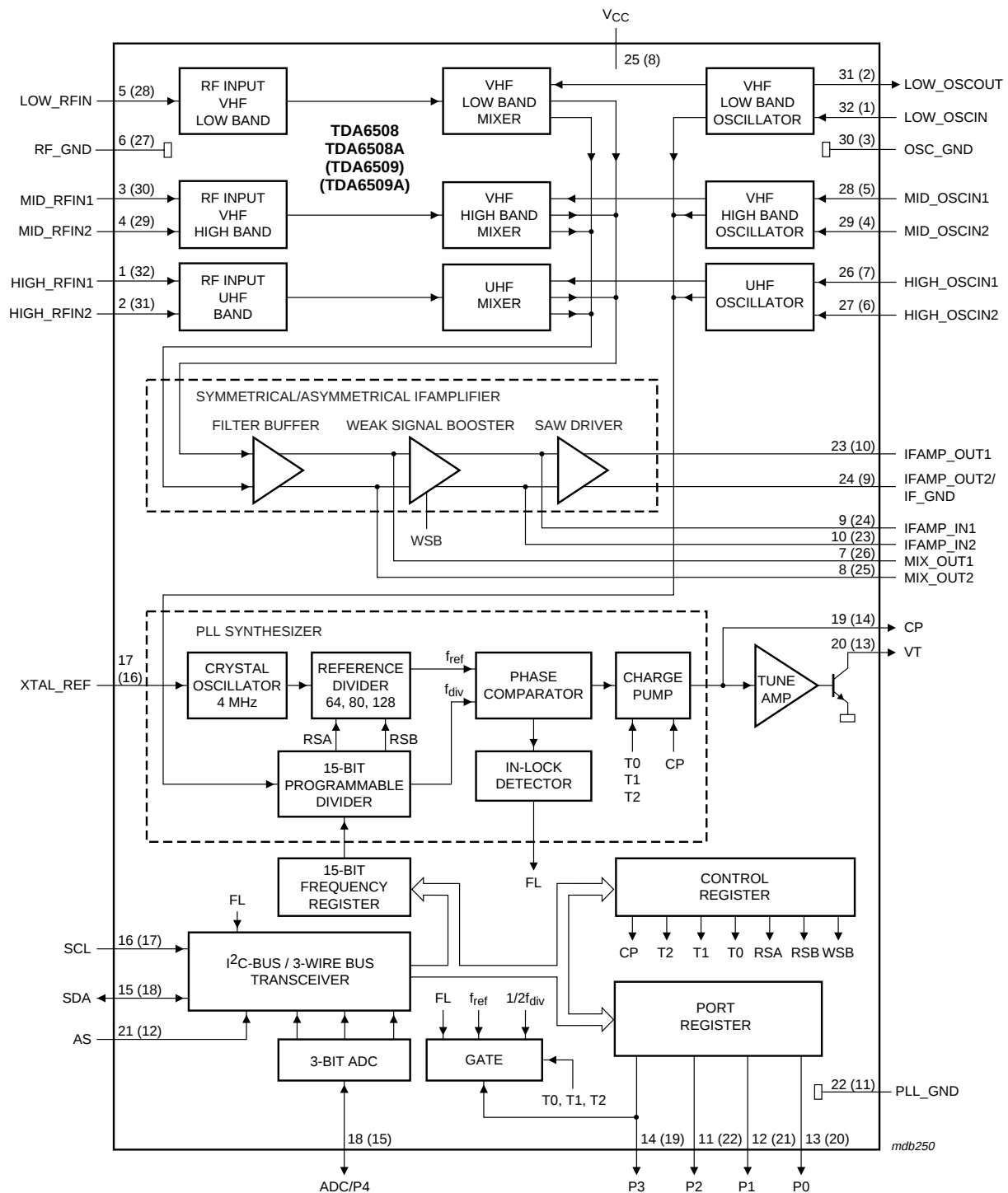
Fig.1 Block diagram.
