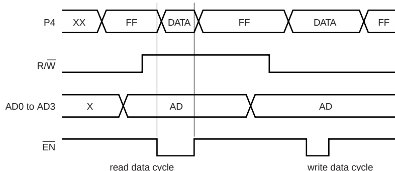
Fig.5 Use of peripheral interface.
