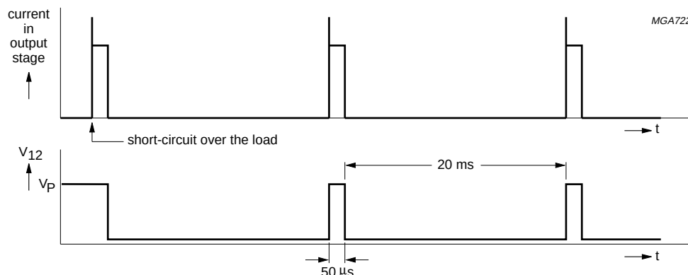
Fig.4 Short-circuit waveform.
