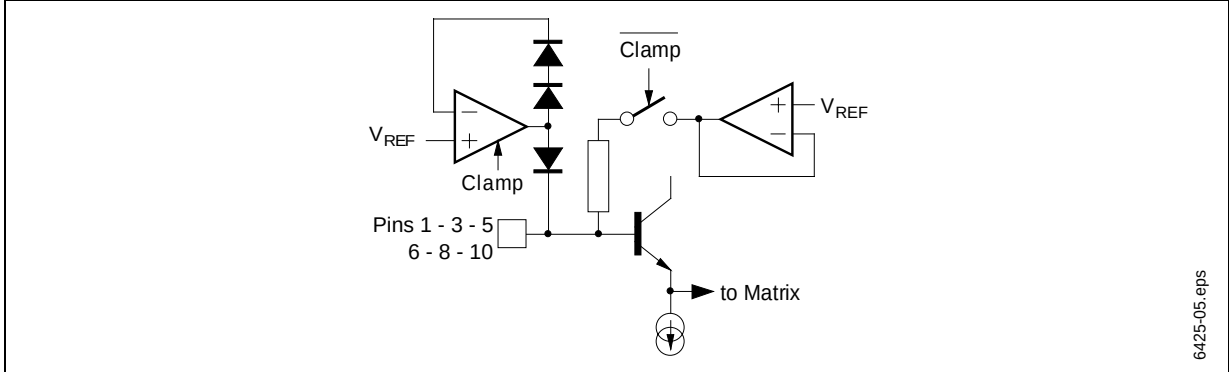
Figure 6. Video OUT
