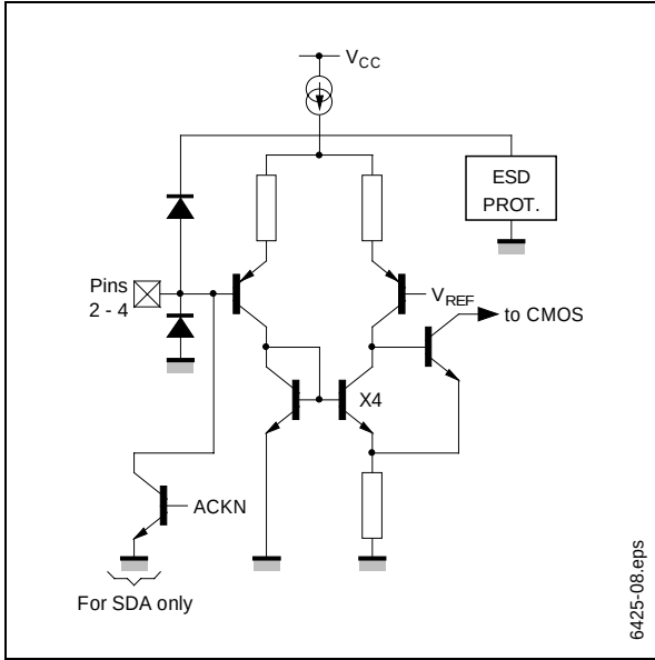
Figure 8. Bus Inputs
