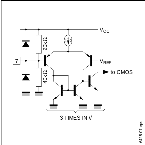
Figure 7. PROG Pin
