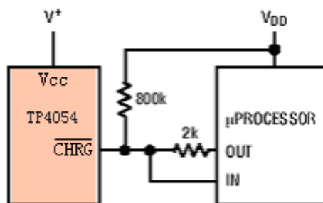
Figure 5. Using a Microprocessor to Determine \overline{CHRG} State
