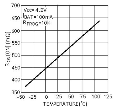
power TEF "ON" Resistance vs Temperature
