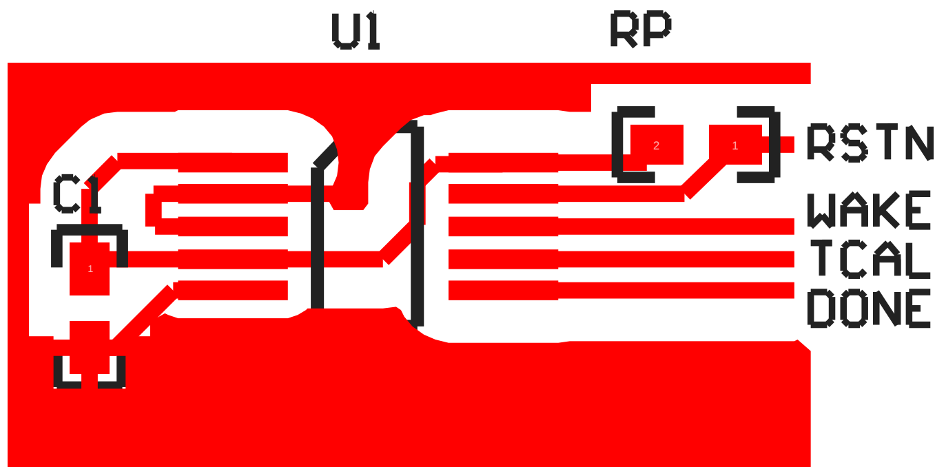
Figure 10. PCB Layout
