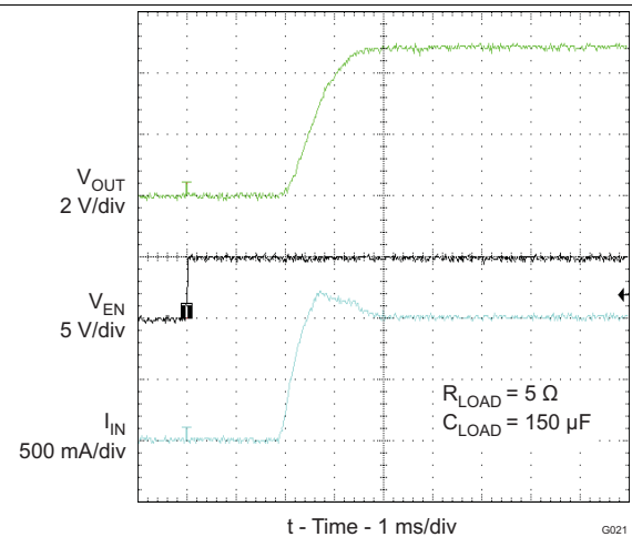
Figure 18. Turnon Response
