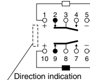
2-coil latching
