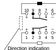
2-coil latching
