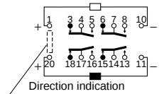
2-coil latching
