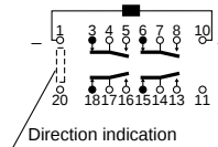
1-coil latching
