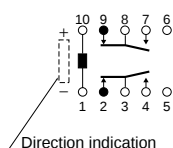
1-coil latching
