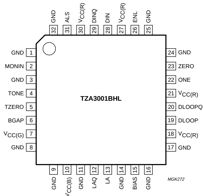
Fig.4 Pin configuration of TZA3001BHL.
