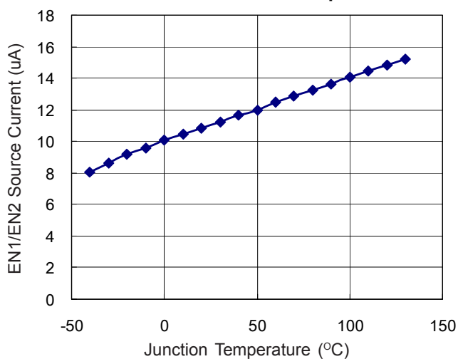
EN1/EN2 Current vs. Temperature
