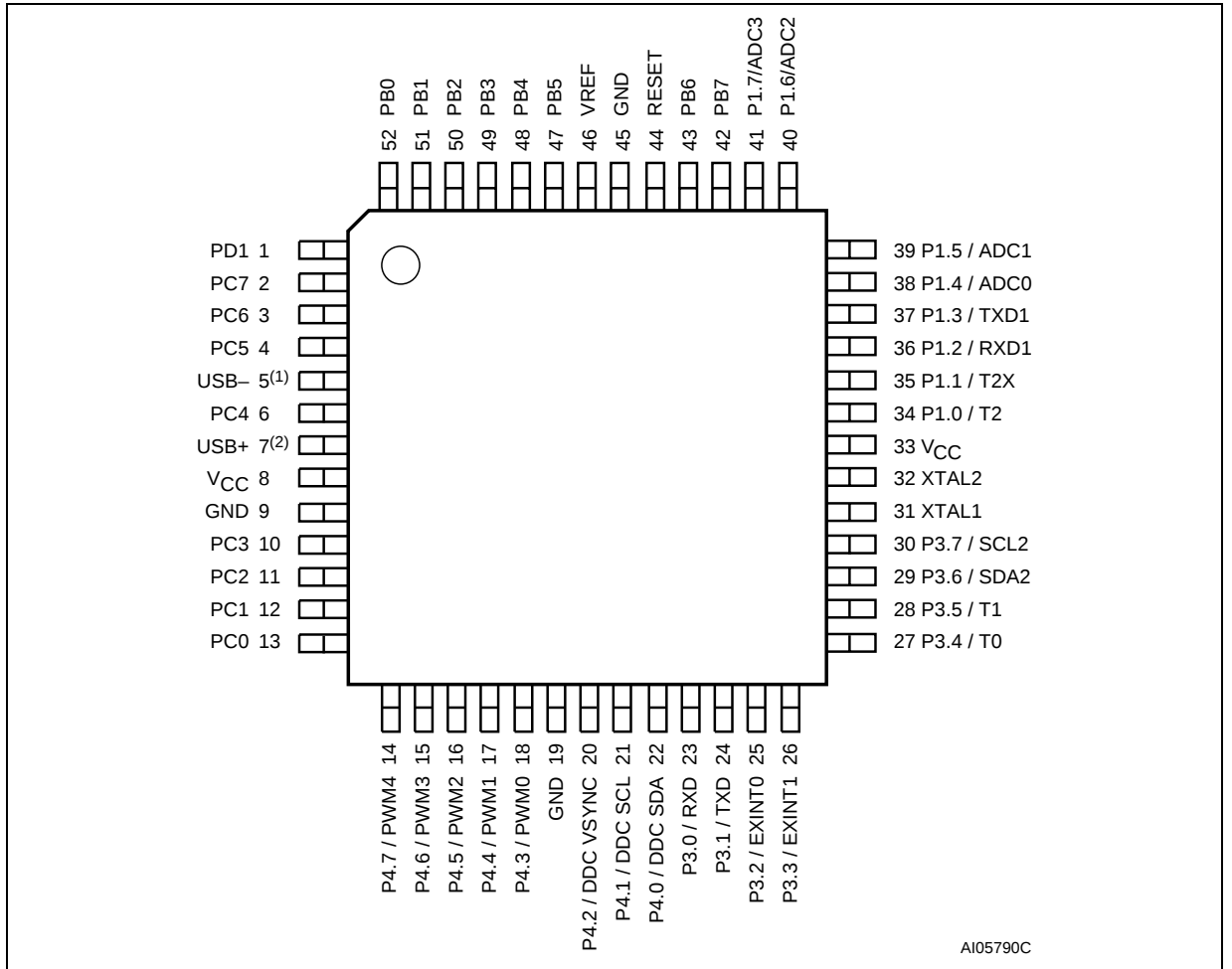
Figure 3. TQFP52 Connections
