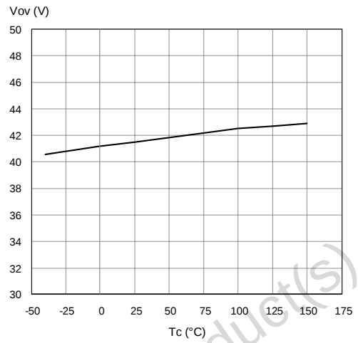
Figure 25. Overvoltage Shutdown
