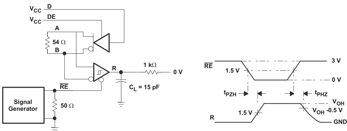
Figure 17. Receiver Enable and Disable Test Circuit and Waveforms, Data Output High
