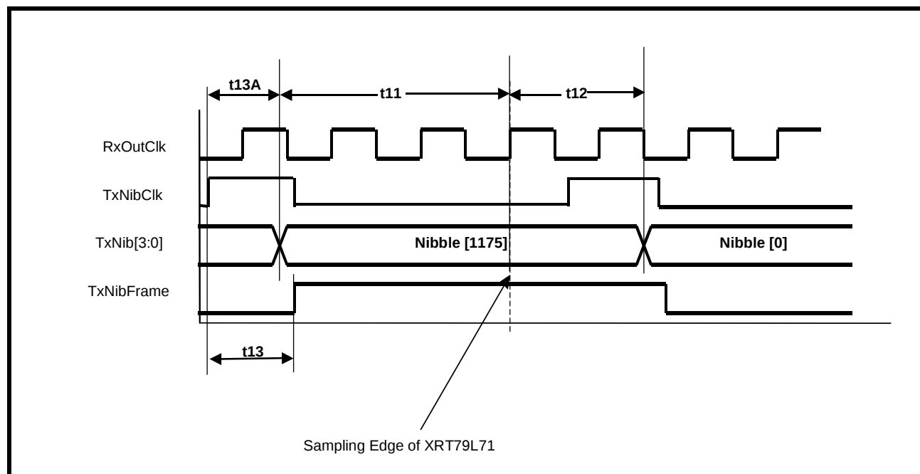
FIGURE 19. TIMING DIAGRAM FOR THE TRANSMIT PAYLOAD DATA INPUT INTERFACE WHEN THE XRT79L71 IS OPERATING IN BOTH THE DS3/NIBBLE-PARALLEL AND LOOP-TIMING MODES
