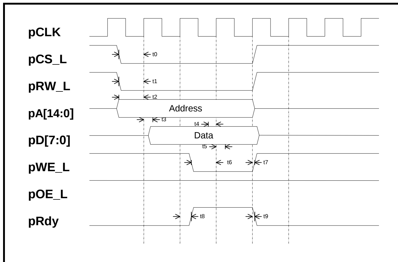
FIGURE 10. SYNCHRONOUS MODE 3 - IBM POWERPC 403 INTERFACE TIMING (WRITE CYCLE)
