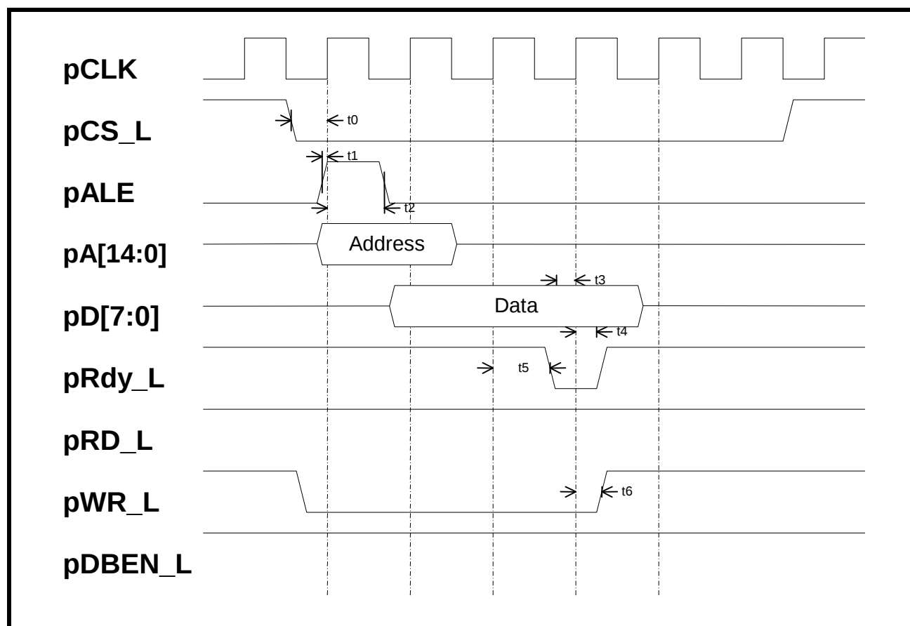
FIGURE 12. SYNCHRONOUS MODE 4 - IDT 3051/52 INTERFACE TIMING (WRITE CYCLE)
