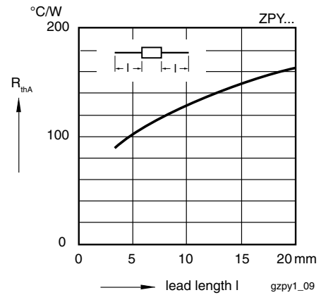
Fig. 5 - Thermal Resistance vs. Lead Length
