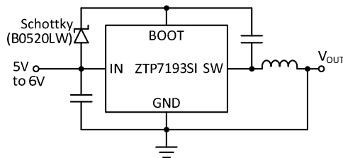
Figure 2: Add a Schottky diode to promote efficiency when V_{\text{IN}} \leq 6\text{V} .
