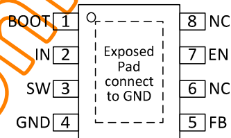
Top View (with EP)
